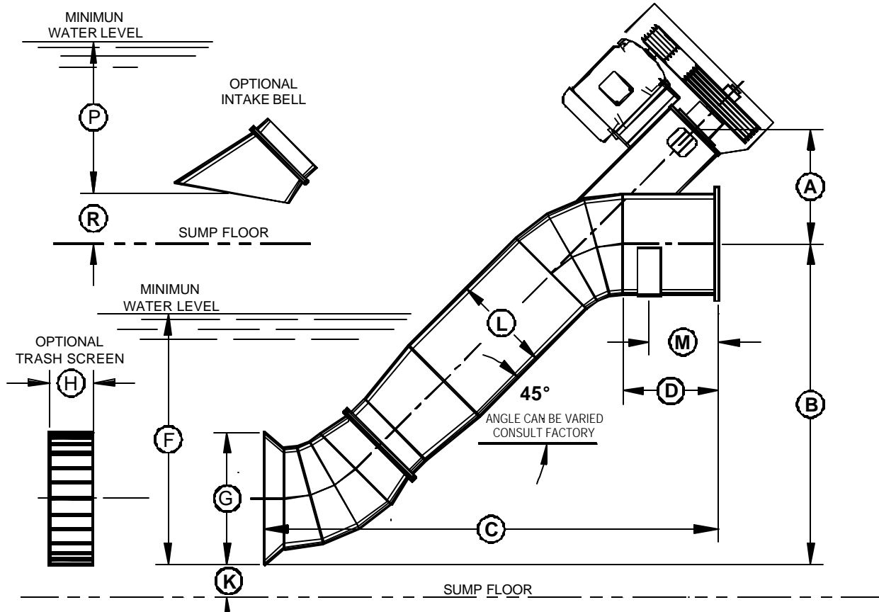
STANDARD DIMENSIONS IN INCHES
