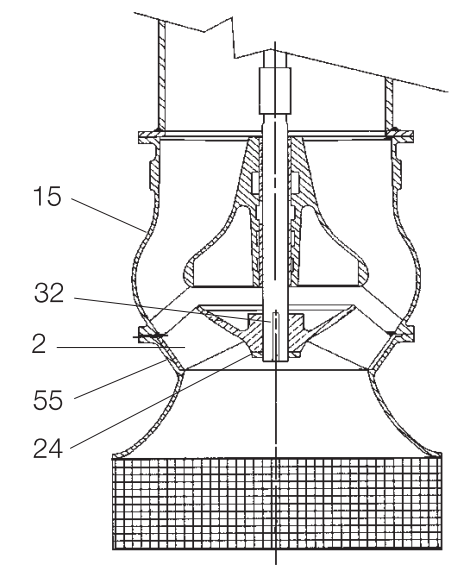
Without bearing below impeller
